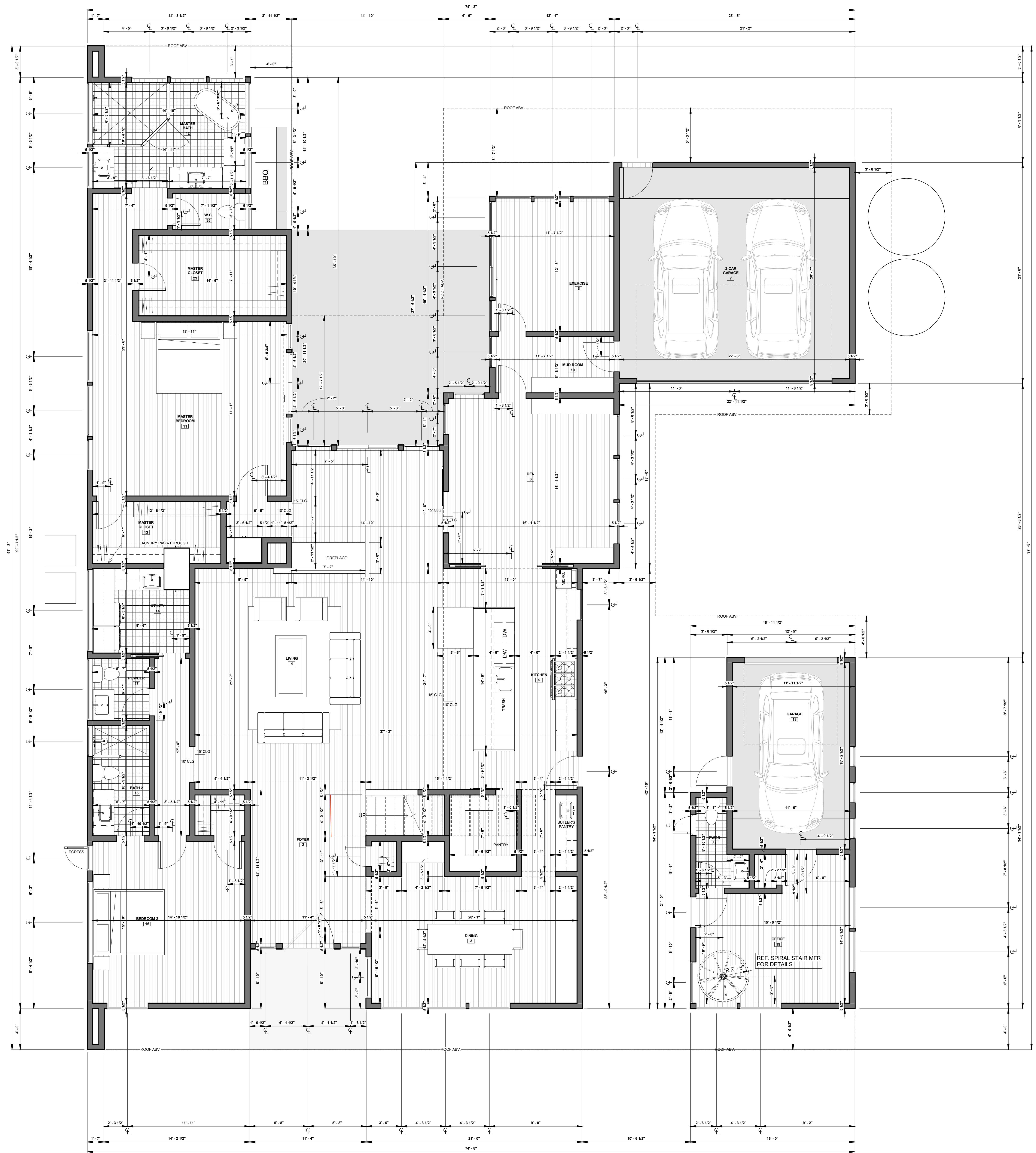
1 A-LEVEL 1 DIMENSION PLAN 1/4" = 1'-0"
